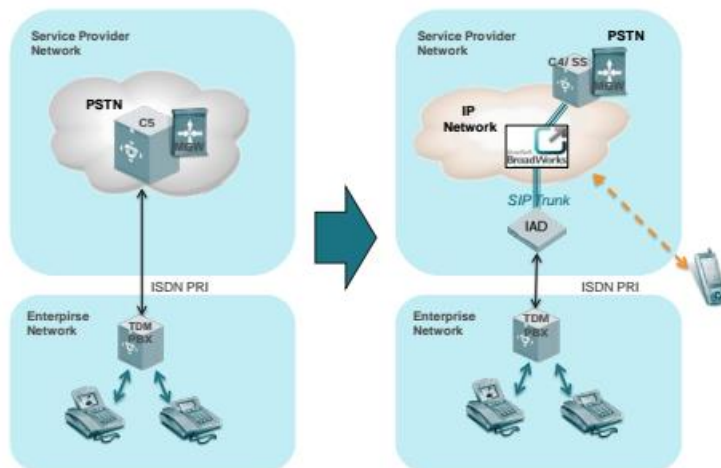
Figure 6: Legacy to Converged VoIP Platform Transition, using IAD illustration
