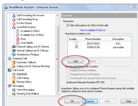
Figure 4: Anywhere example
