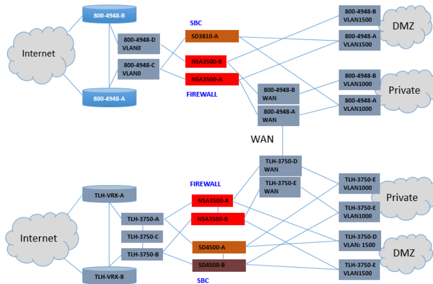
Figure 2: VoIP Logic Network Resiliency visualization
